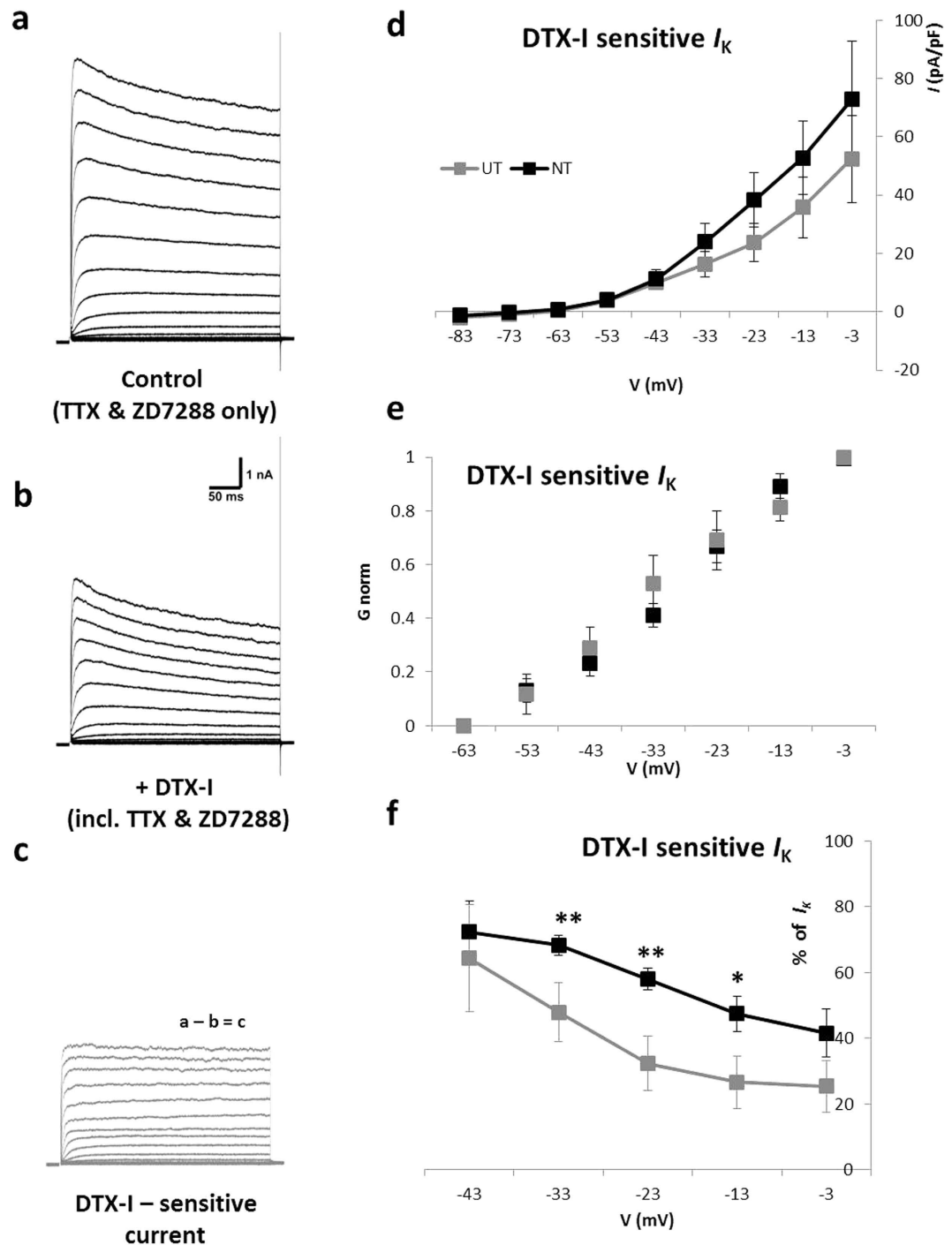
Figure 4. DTX-I sensitive currents in SGNs. (a) Typical outward currents evoked in the absence of sodium and hyperpolarisation-activated currents (example shown is an NT neuron). (b) A reduction in outward currents was observed in the presence of DTX-I. (c) DTX-I sensitive component of the current as determined by the subtraction of recordings in (b) from those in (a). (d) Current-density versus voltage for the sustained portion of the DTX-I sensitive current showed no difference between UT ( n = 6 ) and NT ( n = 7 ) neurons below 0 mV. (e) Normalised conductance-voltage plots depict the activation of the DTX-I sensitive component in each condition. Conductance calculated from the steady-state DTX-I sensitive current fitted. (f) DTX-I sensitive current expressed as a percentage of the overall current. UT – untreated; NT – neurotrophin-treated; * p < 0.05 ** p < 0.01 .
