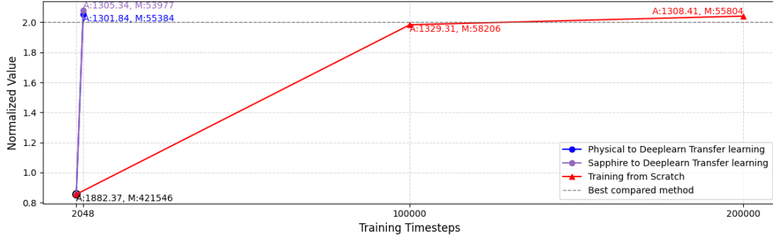
FIGURE 6.4: Comparison of transfer learning performance against training from scratch, showing normalized values of maximum and average waiting times by best performed Heuristics. \text{Normalized Value} = \frac{\text{best\_heuristic}_{\text{avg}}}{\text{model\_waiting\_time}_{\text{avg}}} + \frac{\text{best\_heuristic}_{\text{max}}}{\text{model\_waiting\_time}_{\text{max}}} .
