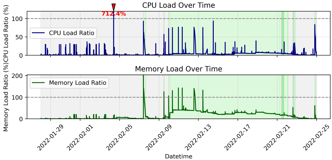
FIGURE 5.6: MetaPilot's action in testing set. Requested CPU and Memory Load in the queue, normalized by the total available resources in the cluster. Shaded regions represent MetaPilot's scheduling decisions: gray indicates optimization for waiting time reduction, while green represents prioritization of resource utilization maximization.
