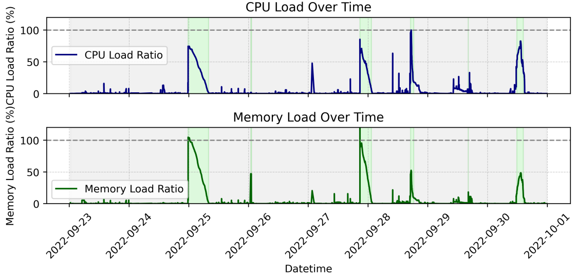
FIGURE 5.5: MetaPilot's action in training set. Requested CPU and Memory Load in the queue, normalized by the total available resources in the cluster. Shaded regions represent MetaPilot's scheduling decisions: gray indicates optimization for waiting time reduction, while green represents prioritization of resource utilization maximization.
