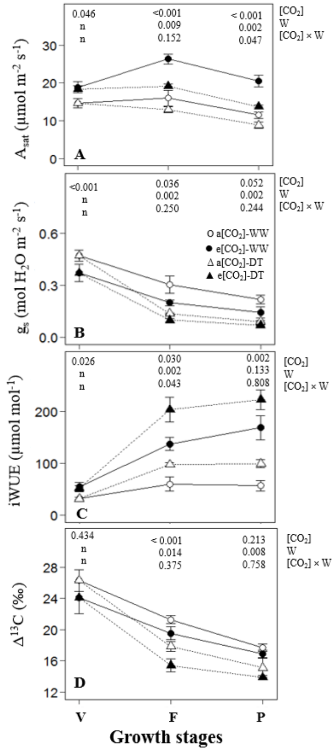
Fig. 5. 3 Light saturated \text{CO}_2 assimilation rate ( A_{sat} , A), stomatal conductance ( g_s , B) and intrinsic water use efficiency (iWUE, C) and ^{13}\text{C} discrimination ( \Delta^{13}\text{C} , D) in leaves of faba bean grown under ambient [\text{CO}_2] ( a[\text{CO}_2] , \sim 400 \mu\text{mol mol}^{-1} ; white bars) and elevated [\text{CO}_2] ( e[\text{CO}_2] , \sim 550 \mu\text{mol mol}^{-1} ; grey bars) and two water (W) regimes (WW: well-watered and DT: drought) and measured at vegetative (V), flowering (F) and pod filling (P) stages. Means and \pm\text{SE} (n=4) in each bar. P-values of the effect of [\text{CO}_2] , water regime (W) and their interactions are shown.
