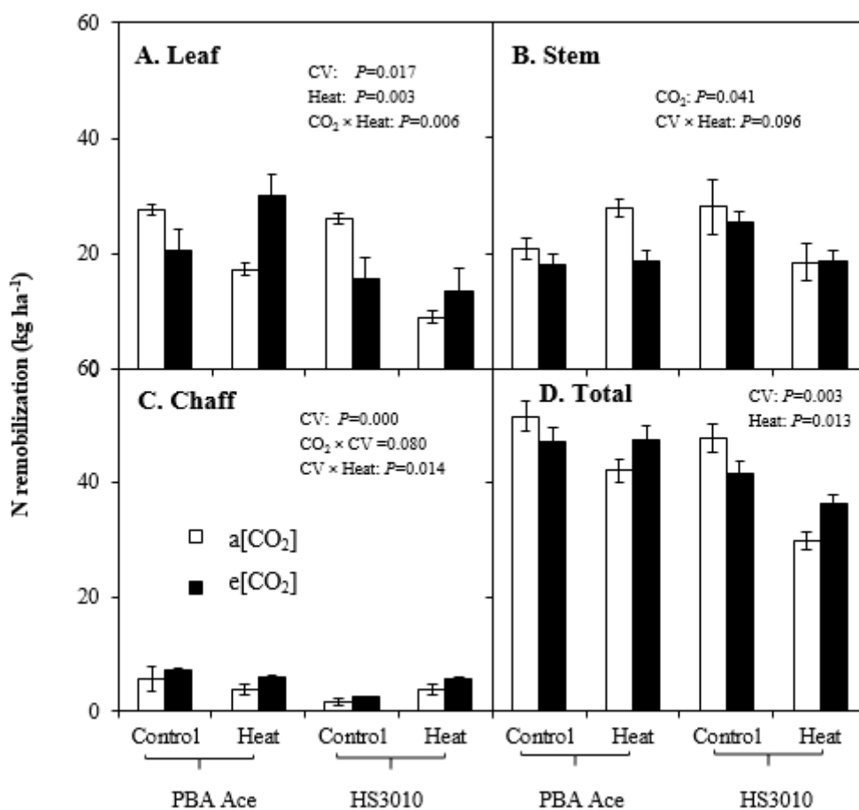
Fig. 6. 5 N remobilization ( \text{kg ha}^{-1} ) in leaf (A), stem (B), chaff (C) and total (D) of two lentil genotypes measured at physiological maturity (R8) stages grown under ambient [ CO_2 ] (a[ CO_2 ], \sim 400 \mu\text{mol mol}^{-1} ) or elevated [ CO_2 ] (e[ CO_2 ], \sim 550 \mu\text{mol mol}^{-1} ) in the Australian Grains Free Air Enrichment (AGFACE) facility, Horsham, Australia. Arrow represents R4 stage when heat shocked was imposed. Data points represent mean values and standard errors of n=4 replicates. Open bars for ambient [ CO_2 ], filled bars for elevated [ CO_2 ].
