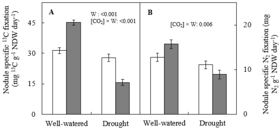
Fig. 7. 7 Nodule specific ^{13}\text{C} fixation (A) and specific \text{N}_2 fixation (B) of faba bean grown under a[ \text{CO}_2 ] (~400 \mu\text{mol mol}^{-1} , white bars) or e[ \text{CO}_2 ] (~700 \mu\text{mol mol}^{-1} , grey bars) and two water (W) regimes (well-watered and drought) and harvested at 60 DAS. Means and \pm\text{SE} (n=8) in each bar. Only significant relations ( P<0.05 ) are shown.
