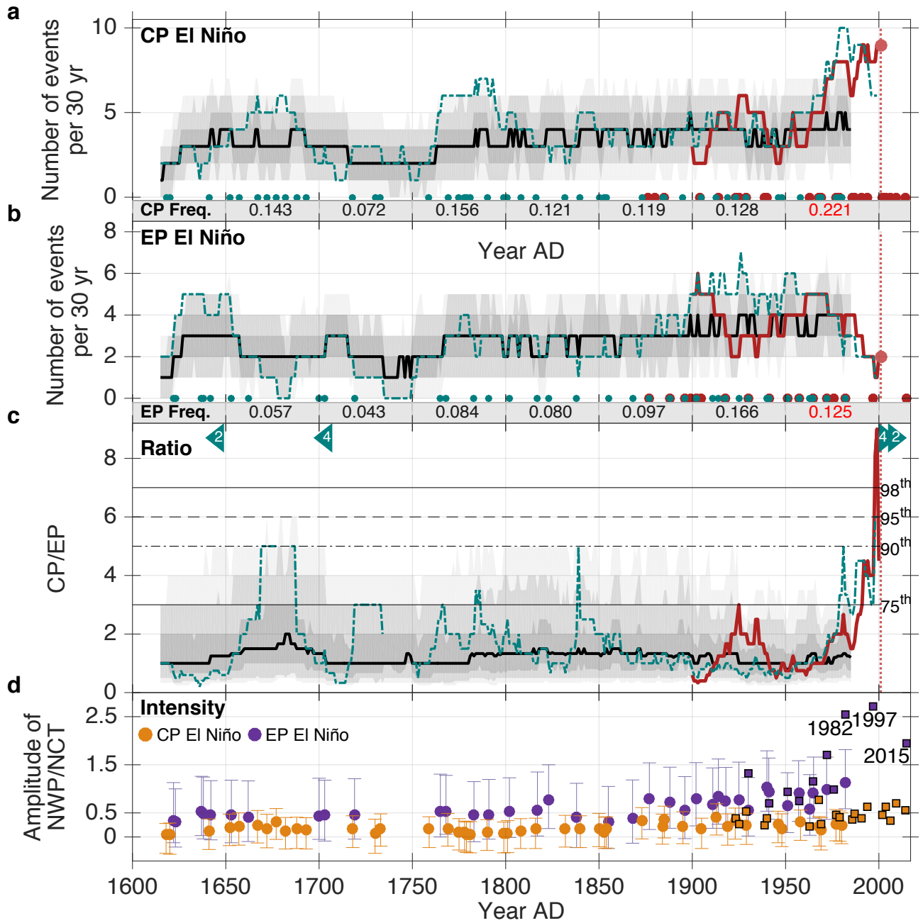
Figure 4: El Niño event diversity over the past four centuries. a,b,c , Number of CP El Niño ( a ), EP El Niño events ( b ) and ratio of CP to EP events ( c ) in sliding 30-yr windows; instrumental (red), most-replicated reconstruction (teal), bootstrapped median (black) and uncertainty range in grey shadings (75 th , 90 th , 95 th percentiles) shown. Event occurrence frequencies (per decade, insets) in 50-yr periods; individual events indicated by markers at zero line. Vertical red dotted line indicates most recent window, centred on 2001. d , Intensity of CP and EP El Niño events obtained by the NWP/NCT indices; instrumental events outlined in black; error bars indicate 95% confidence interval from bootstrapping. Small triangles show the number of contributing records when data availability is limited.
