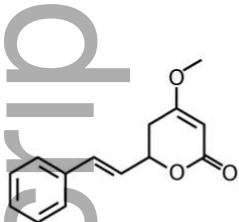
KAWAIN
