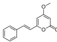
DESMETHOXY YANGOIN
